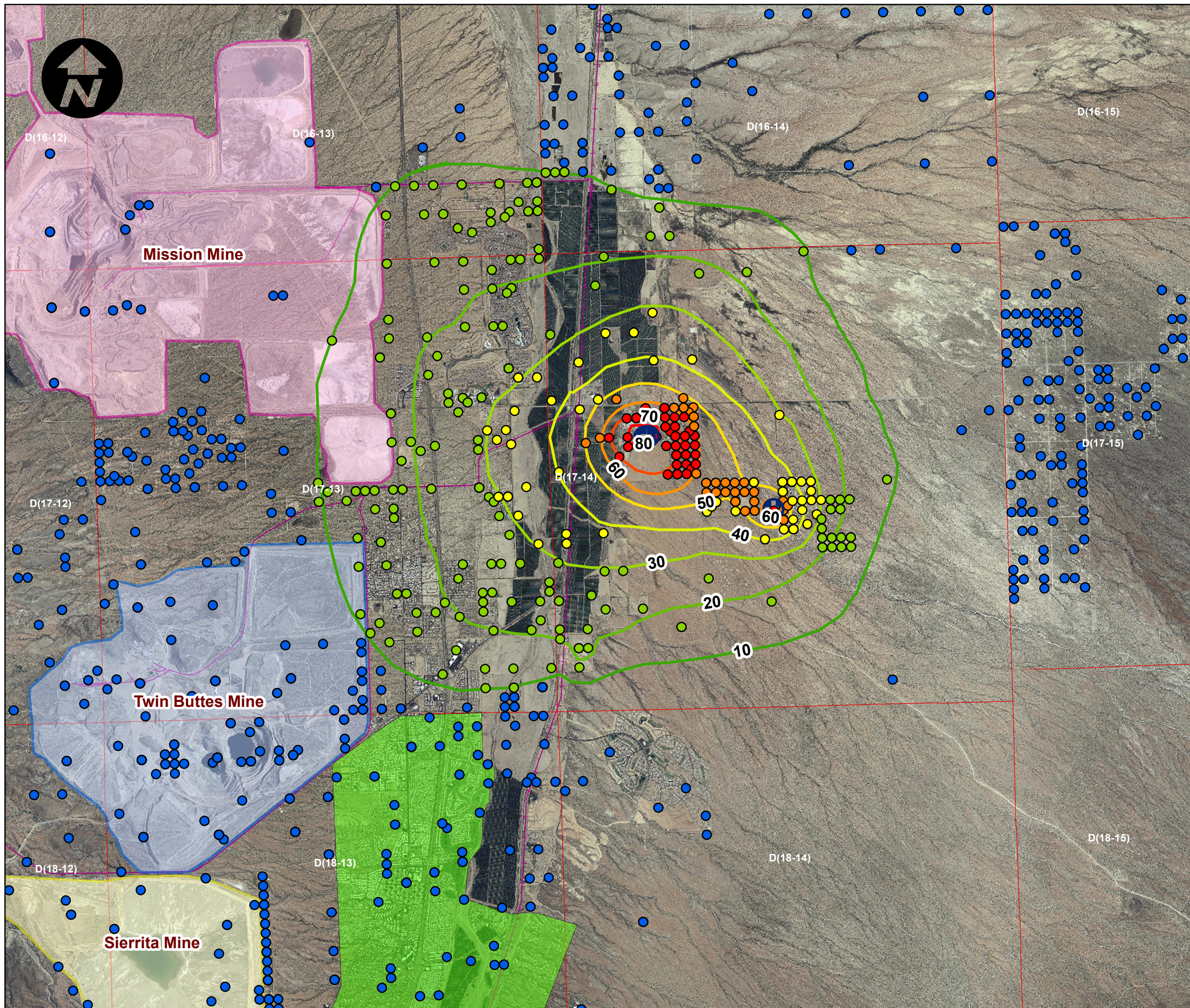
Figure 1 Draft EIS Review Rosemont Copper Project Estimated Drawdown after 20 Years January 2012
